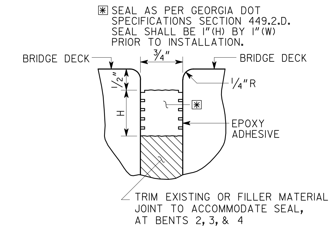
EXPANSION JOINT DETAILS NO SCALE
