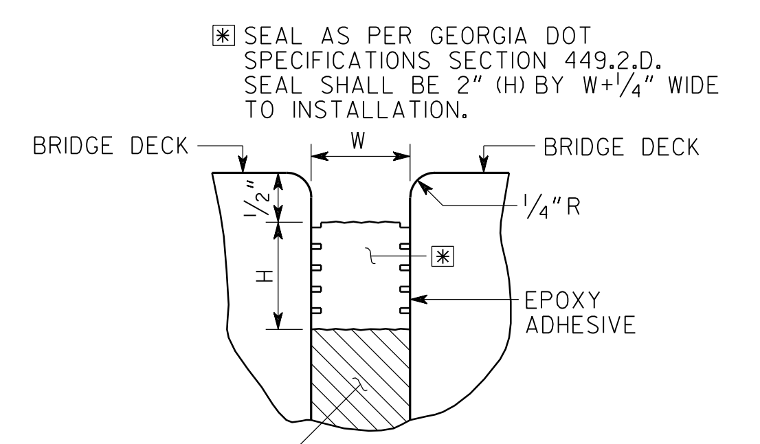
EXPANSION JOINT DETAILS NO SCALE
